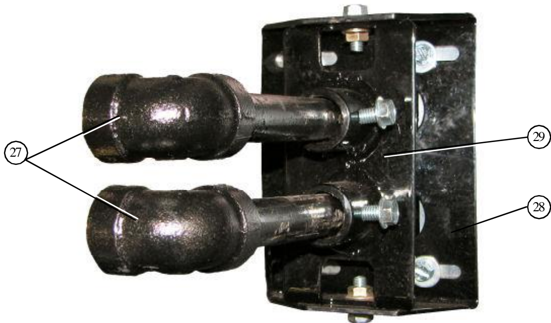
36" Vaporizer coil connection and adjustment brackets.
